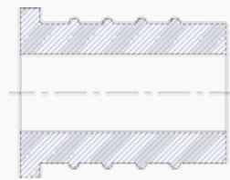
Rubber Plug to hold cable in HDPE subduct.
