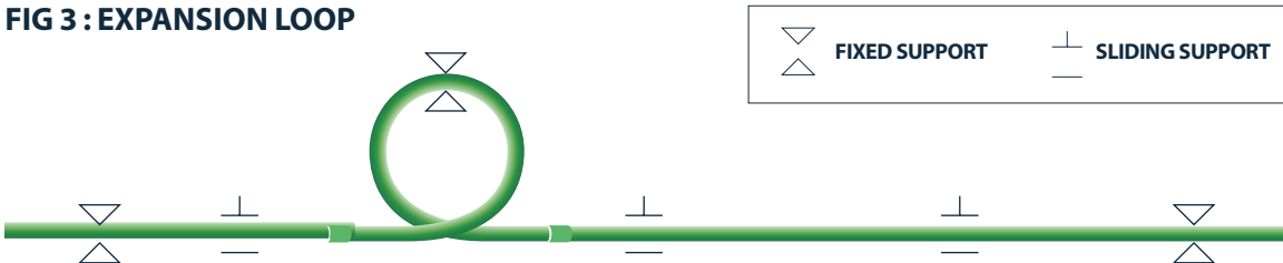
FIG 3: EXPANSION LOOP
