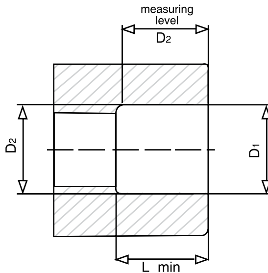
Figure 1 - Dimensions of socket weld fittings
