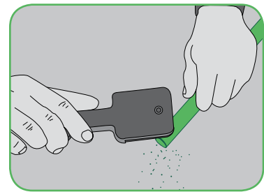
FIG. 3 Scrap the marked end of the pipe to remove the thin seduction layer using the mark as a stop point. Wipe the scrapped area and the electrofusion fitting with an alcohol stuched paper towel.
